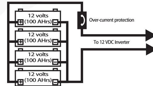
12 volt battery bank (total capacity = 400 Ahrs) Figure 5, Parallel Battery Wiring
