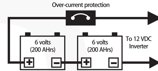
12 volt battery bank (total capacity = 200 Ahrs) Figure 4, Series Battery Wiring
